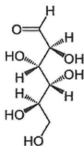
D-mannose
